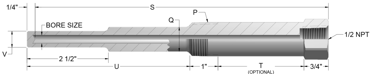
Thermowell Dimensions
